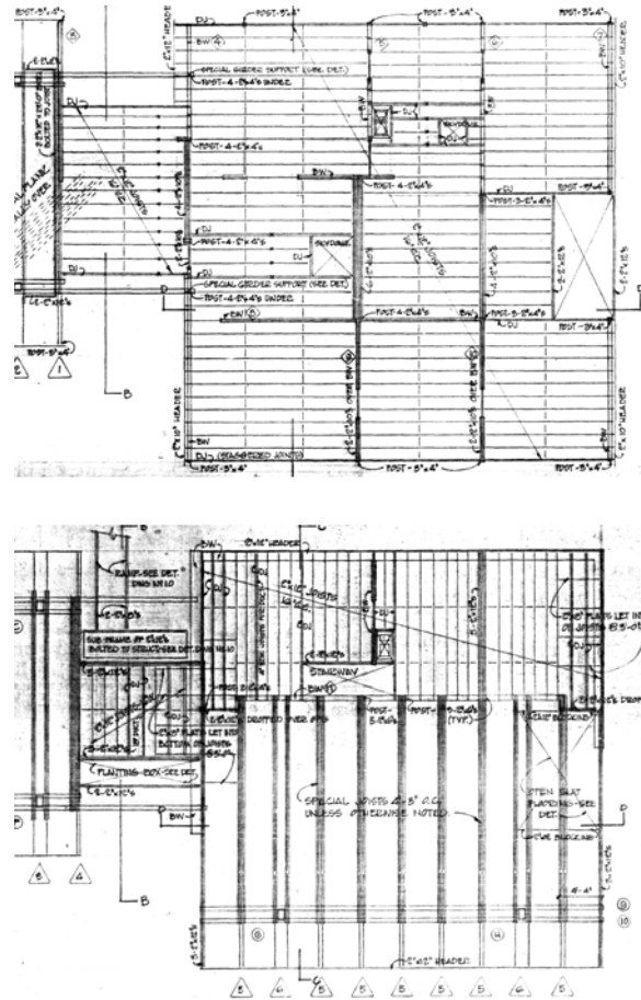
Figure 2: Starkey House Framing Plans
